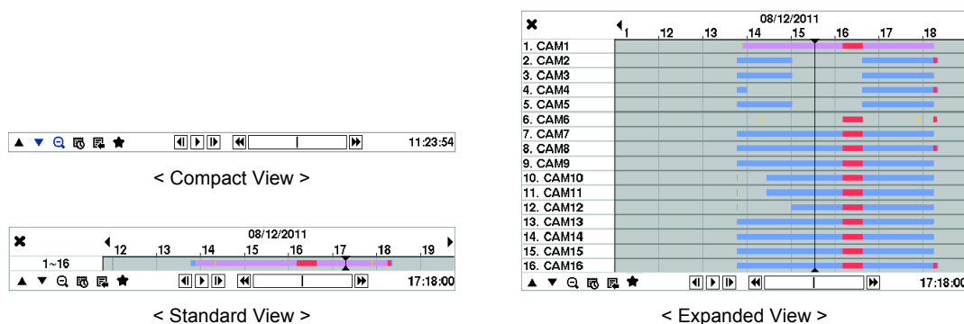
Figure 71 — Record Table Search screen.
