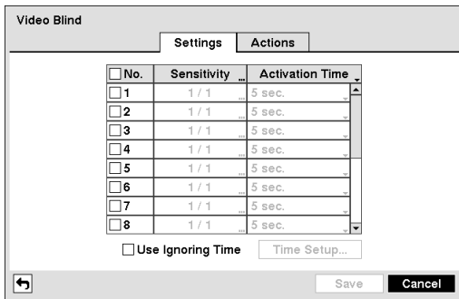
Figure 35 — Video Blind Settings screen.
