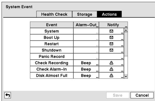
Figure 42 — System Event Actions screen.
