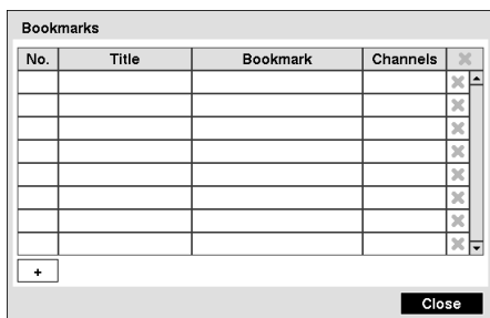
Figure 75 — Bookmarks screen.
