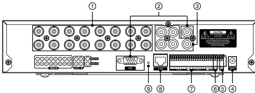
Figure 2 — DVR rear panel.
