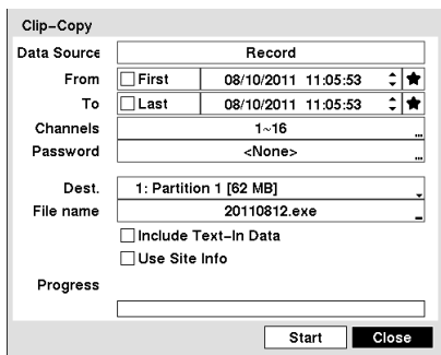
Figure 76 — Clip-Copy screen.
