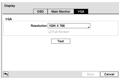
Figure 63 — VGA screen.
