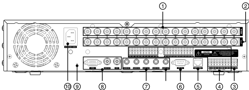
Figure 2 — 16-Channel DVR rear panel.
