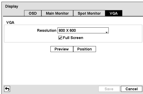
Figure 67 — VGA screen.
