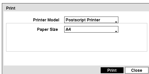
Figure 82 — Print screen.
