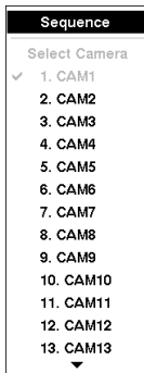
Figure 72 — Sequence menu.
