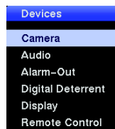
Figure 57 — Devices menu.
