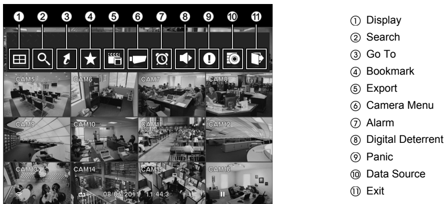
Figure 74 — Search menu.
