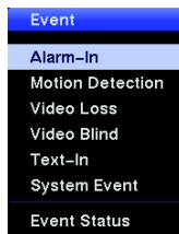
Figure 26 — Event menu.
